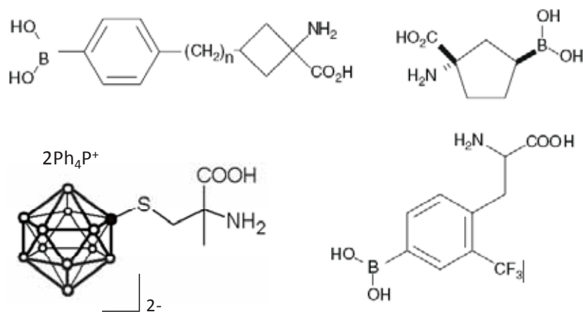
Figure 1.3. Structures of boron-containing amino acids. In the cluster, white dots stand for B-H; black dot stands for B.
