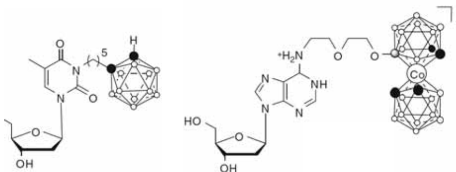
Figure 1.4. Structures of boron-containing nucleic acids. In the cluster, white dots stand for B-H; black dots stand for C (left) or C-H (right); grey dot stands for B.
