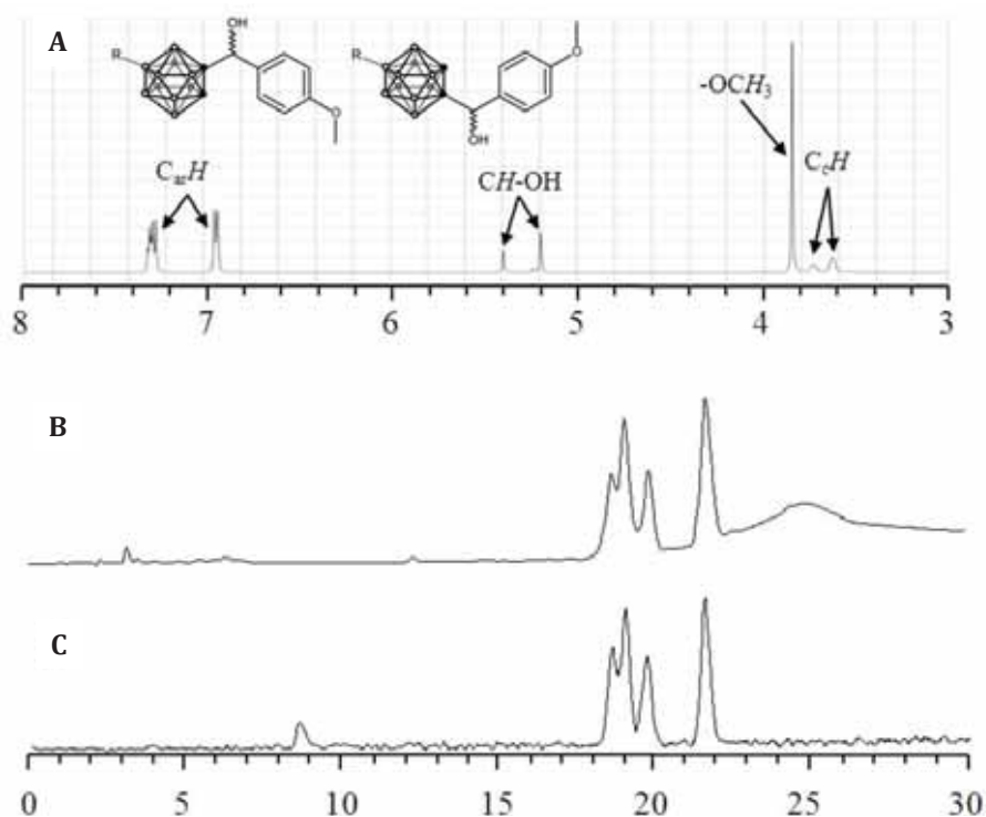
Figure 4.6. (a) ^1\text{H}\{^{11}\text{B}\} -NMR spectrum of 4.5 ; (b) HPLC profile of 4.5 (UV detector) and [^{18}\text{F}]\text{4.5} (radiometric detector) obtained using a chiral column.
