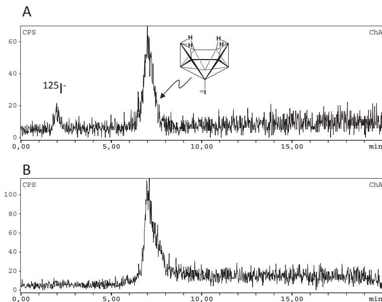
Figure 4.9. Chromatographic profiles (radiometric detection) for: (A) reaction crude and (B) pure 1- ^{125}\text{I} decaborane.
