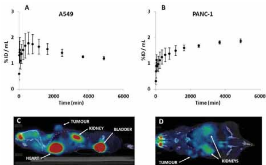
Figure 5.10. Biodistribution of [ 18 F]FDG in subcutaneous PANC-1 (human pancreatic carcinoma) and A549 (carcinomic human alveolar basal epithelial cell line) xerograft mouse models. Time-activity-curves in the tumour, expressed as the percentage of the injected dose (%ID) per cm 3 of tissue are shown in (A) and (B). PET sagittal (C) and coronal (D) slices resulting from averaged images (frames 5-15) obtained after administration of [ 18 F]FDG in mice bearing A549 (C) and PANC-1 (D) tumours are shown; optimal view-point and slides were selected for correct visualization of the tumour.
