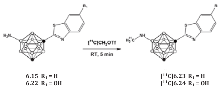
Figure 6.7. Schematic reaction for the preparation of [\text{11C}]\text{6.23} and [\text{11C}]\text{6.24} using [\text{11C}]\text{CH}_3\text{OTf} as the labelling agent.
