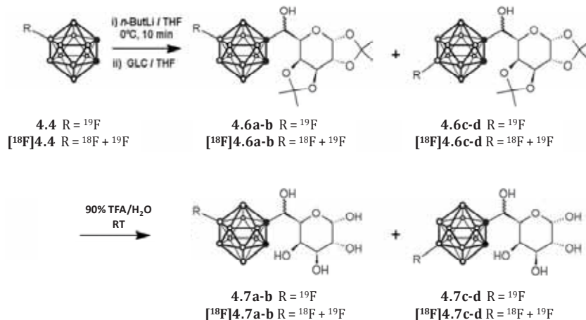
Figure 4.7. syntheses of ^{19}\text{F} - and ^{18}\text{F} -labelled \text{C}_c substituted o -carborane by reaction of 9-fluoro- and 9- ^{18}\text{F} -fluoro- o -carborane with 1,2:3,4-di- O -isopropylidene- \alpha -D-galactohexadialdo-1,5-pyranose and hydrolysis.
